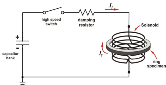
Fig. 2. Schematic diagram of the arrangement for electromagnetic ring expansion.
